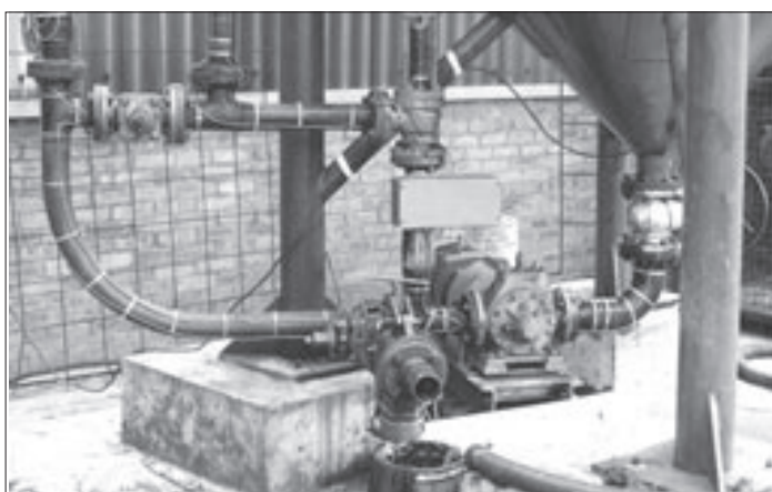
Trace Heating of Industrial Pipework carrying Grease
