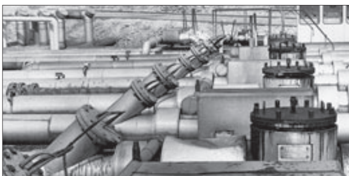
Fuel Oil Pipework fitted with Internal Heating Cable
